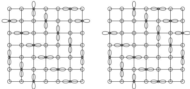
Figure 1.14. Left: single stripes (“Wigner crystal”). Right: paired stripes, or bistripes in \text{La}_{1-x}\text{Ca}_x\text{MnO}_3 for x = \frac{2}{3} . \text{Mn}^{4+} ions denoted by O and \text{Mn}^{3+} ions by 8, \infty .
