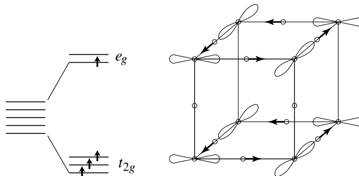
Figure 1.2. Left: splitting of 3d -levels in a cubic crystal field (regular \text{MnO}_6 -octahedron). Electron occupation of the four 3d -electrons in \text{Mn}^{3+} is shown by arrows. Right: orbital ordering of \text{LaMnO}_3 . Arrows indicate the displacements of oxygen ions.
