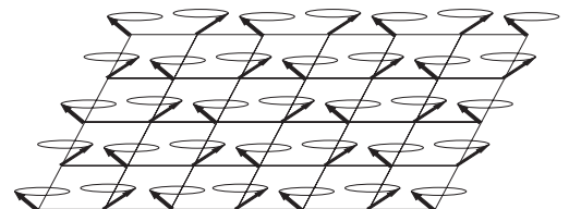
Fig. 1. A schematic representation of the groundstate of the local pairing superconductor on a square lattice. The arrows are semiclassical representations of the pseudospins \sigma .
