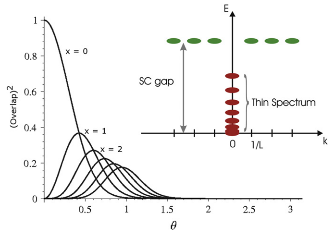
Fig. 2. The overlap between the thin spectrum state |x\rangle and the rotated groundstate \hat{R}(\theta)|0\rangle , as a function of the angle of rotation \theta , for different values of x . To make this graph we used the values J = 10 , B = h = 1 and N = 100 . For higher values of N the graph for each n will be scaled horizontally, but the height of the top remains unaffected. The plot is symmetric under mirroring in the \theta = 0 axis. The inset shows a schematic dispersion relation of the low-energy, low-momentum states of a finite superconductor: the states at finite k are gapped, while the thin spectrum states at k = 0 lie within the gap.
