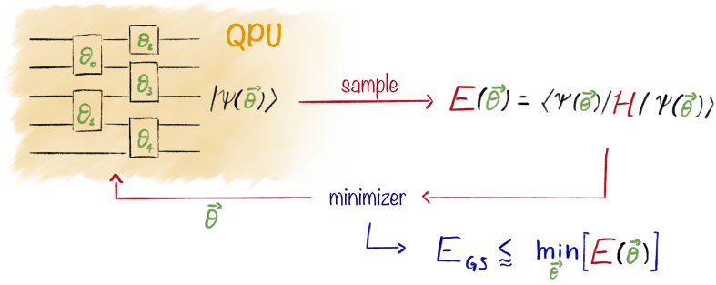
Figure 1.3: Block scheme of the variational quantum eigensolver. The subroutine run on the quantum device (labeled QPU) prepares an ansatz state |\psi(\boldsymbol{\theta})\rangle through a quantum circuit whose gates are parameterized by the elements \theta_j of \boldsymbol{\theta} . The expected energy E(\boldsymbol{\theta}) of |\psi(\boldsymbol{\theta})\rangle is measured by sampling on many repetitions of the circuit, and minimized by a classical outer loop.
