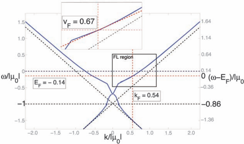
Fig. 3. Maxima in the spectral function as a function of k/\mu_0 for \Delta_\psi = 1.35 and \mu_0/T = -30.9 . Asymptotically for large k the negative- k branchcut recovers the Lorentz-invariant linear dispersion with unit velocity, but with the zero shifted to -\mu_0 . The peak location of the positive- k branchcut that changes into the quasi-particle peak changes noticeably. It gives the dispersion relation of the quasi-particle near (E_F, k_F) . The change of the slope from unity shows renormalization of the Fermi velocity. This is highlighted in the inset. Note that the Fermi energy E_F is not located at \omega_{\text{AdS}} = 0 . The AdS calculation visualizes the renormalization of the bare chemical potential \mu_0 = \mu_{\text{AdS}} to the effective chemical potential \mu_F = \mu_0 - E_F felt by the low-frequency fermions.
